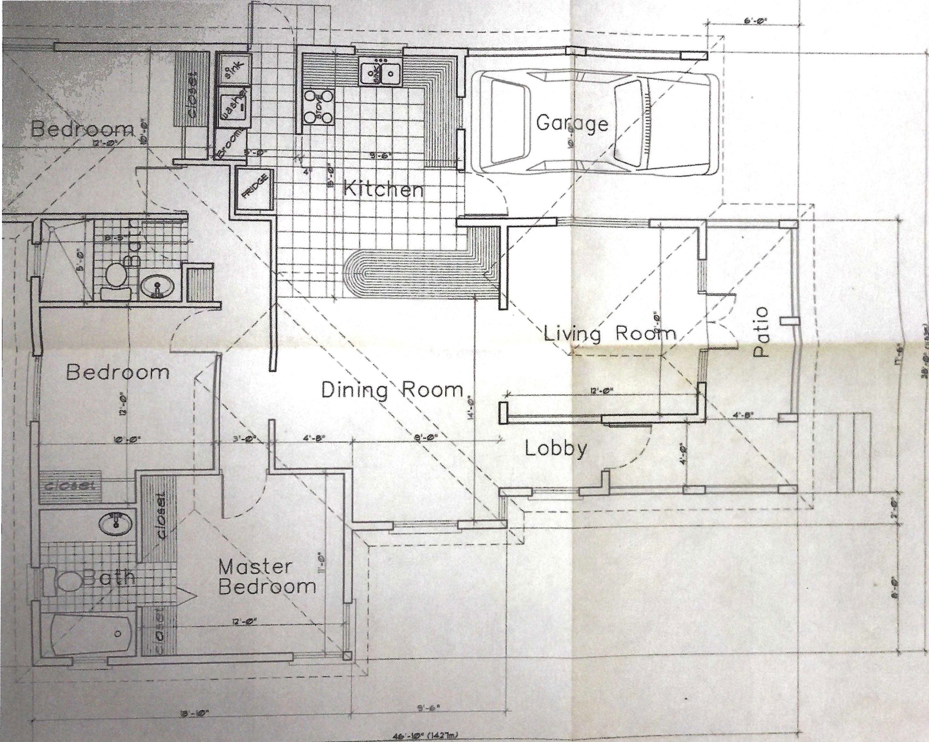
FLOOR PLAN SCALE 1/4" to 1'-0"
